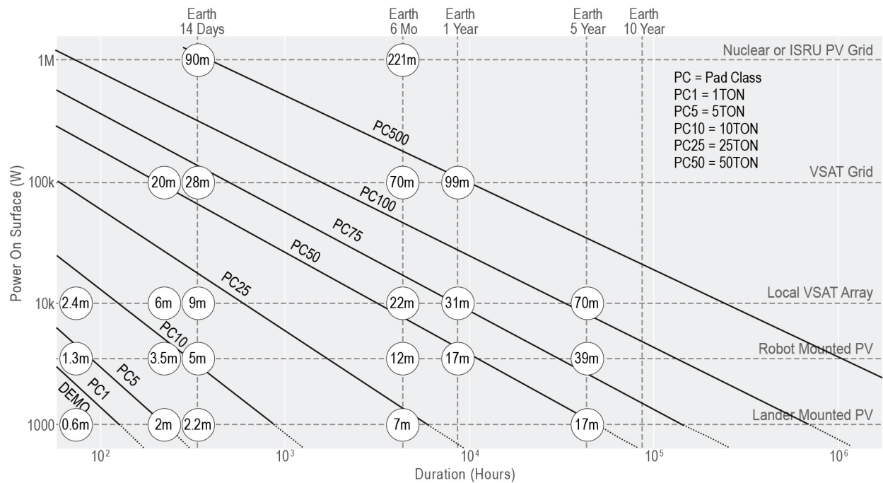
Figure 9.2. Pad production versus power-on surface and time. [Credit: ICON]
