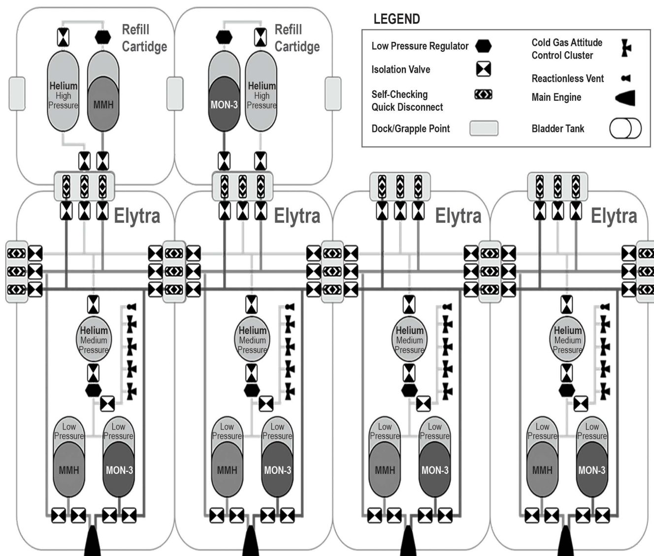
Figure 13.2. Conceptual flow diagram for a networked blowdown system of containerized propellant. [Credit: Firefly Aerospace]
