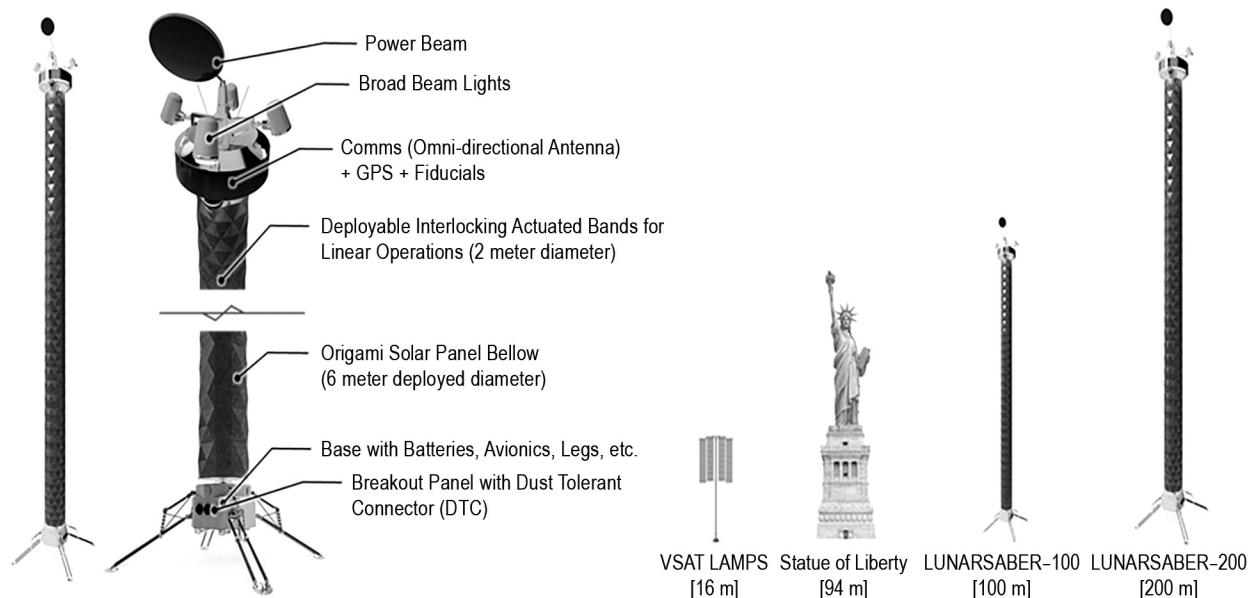
Figure 10.1. (Left) LunarSaber stowed and deployed configurations with subsystem breakdown. (Right) Form factor options. LunarSaber can scale to 100 m and 200 m heights to increase the periods of continuous illumination and shorten periods in darkness. [Credit: Honeybee Robotics]
