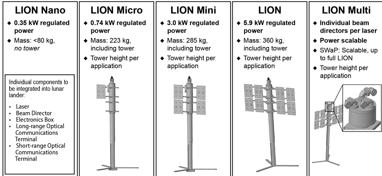
Figure 4.2. LION family of scalable OWPT configurations using a common core subsystem. [Credit: Fibertek]
