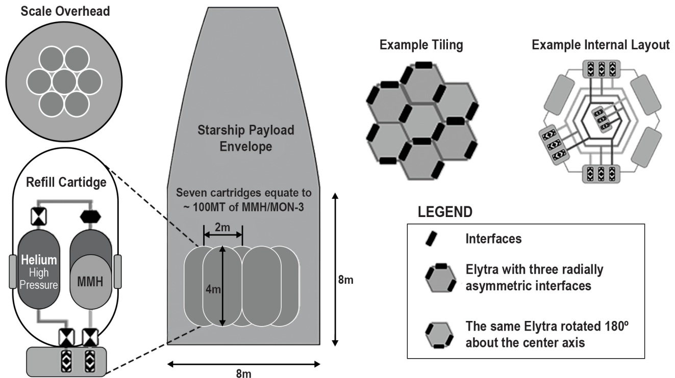
Figure 13.3. (Left) Containerized propellant delivery with 100 MT capacity vehicle. (Right) As few as three interfaces complete a fluid network with no loss of open tiling positions for growth. [Credit: Firefly Aerospace]
