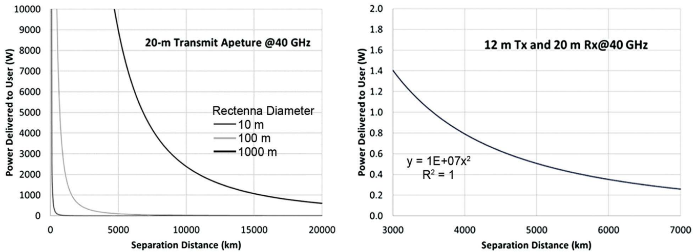
Figure 4.6. Power delivered via RF SBSP is highly sensitive to rectenna size. (Left) Power delivered at Ka-band to a ground-based lunar user as a function of separation distance and rectenna diameter. (Right) Power delivered to user over distance for 1 kWh analysis. [Credit: Redwire Space]
