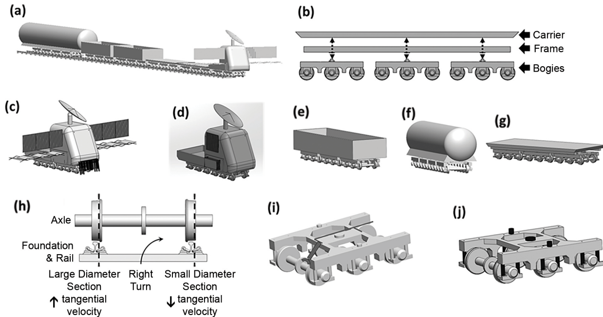
Figure 12.5. Integrated rail vehicles. (a) Example train consisting of an engine, two flatbeds, two hoppers, and a tanker. (b) The construction of a flatbed carrier with bogies, frame, and carrier. The Engine vehicle is shown in (c) day and (d) night mode. Standard hauler carriers are shown: (e) hopper, (f) tanker, and (g) flatbed. (h) Diagram of rail wheel turning. (i) Brake assembly on standard bogie and (j) suspension assembly on standard bogie. [Credit: Northrop Grumman]
