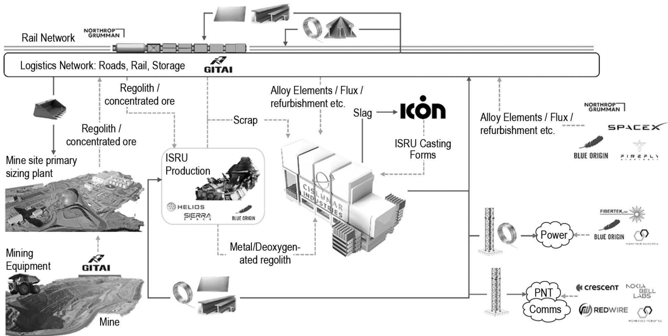
Figure 6.2. Summary of the foundry framework, highlighting external dependencies to other lunar commercial services.
