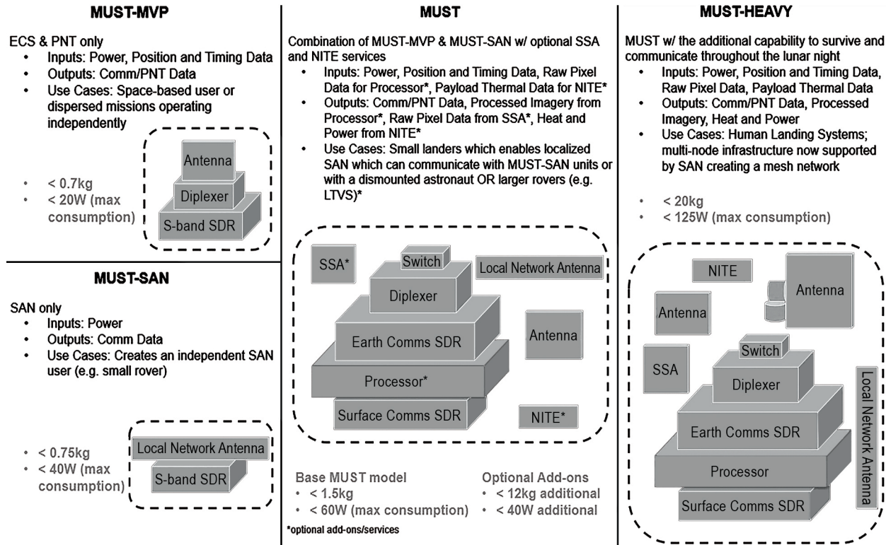
Figure 7.1. Summary of various scalable Comms/PNT commercial units. (Credit: Crescent Space)
