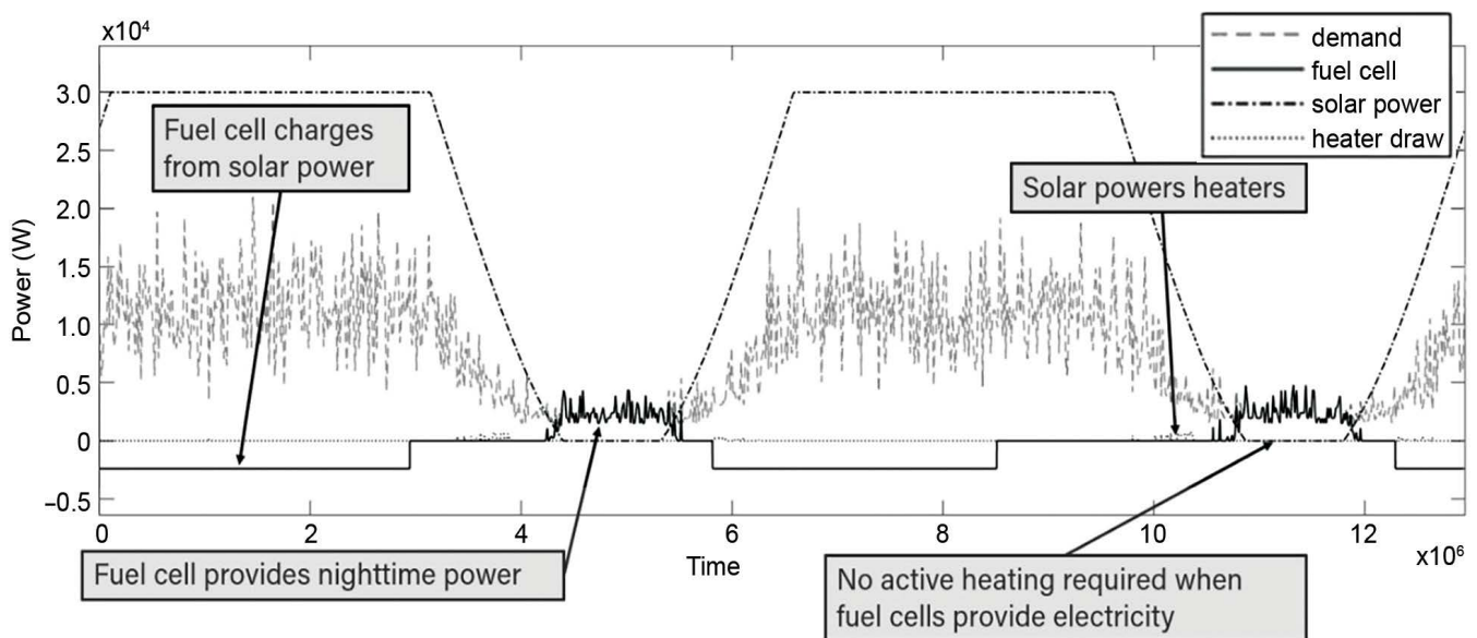
Figure 11.4. Electrical power production and demand of the regenerative fuel cell enhanced Lunar Oasis in a lunar polar region. [Credit: Honeybee Robotics]
