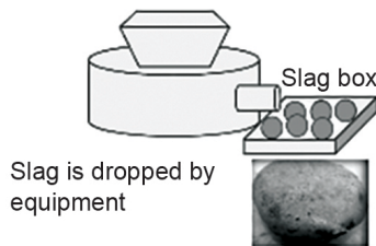
Figure 8.4. Use Case 1, Concept of operations for RaaS-centered ISRU construction and operation, part 2: (top) For regolith loading, the Inchworm can reach both the lunar surface to scoop regolith and the top of the hopper to load the regolith, using grasping fixtures on the lander. (Bottom) For slag removal, the slag dropped by equipment is delivered by Mover robot to a storage location or a potential customer. ICON and CisLunar Industries are notional partners in this process. [Credit: GITAI]
