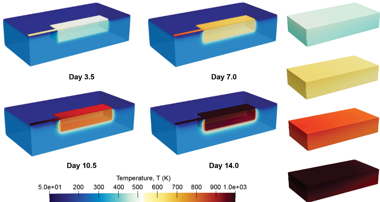
Figure 11.8. Thermal blanket configuration under constant 200 W input power condition. Color contour plot shown of surface temperatures; physical body is section cut. [Credit: ICON]
