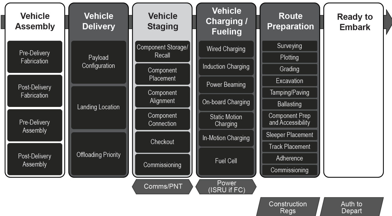
Figure 15.9. Lunar rail transport, task analysis detail, prior to embarking (pre-underway) phase
