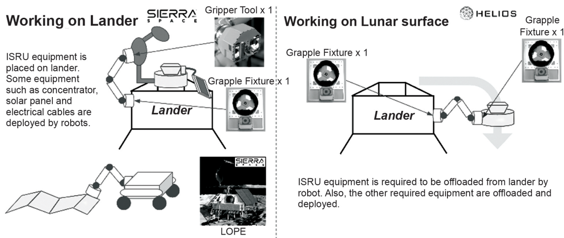
Figure 8.3 Use Case 1, Concept of operations for RaaS-centered ISRU construction and operation, part 1: (left) ISRU equipment is placed on lander. Some equipment, such as concentrator, solar panel, and electrical cables, is deployed by robots. To work on the lunar surface (right), ISRU equipment is offloaded from the lander by robots and placed onto the Mover. The other required equipment is offloaded and deployed. Sierra Space and Helios are notional partners in this process. [Credit: GITAI]
