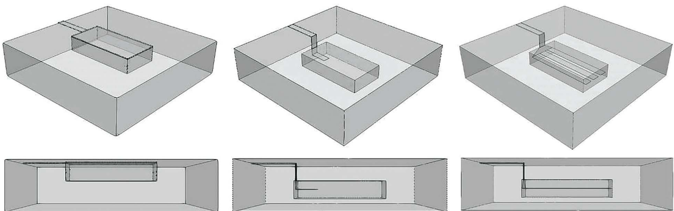
Figure 11.6. System configuration for blanket over exposed VMX mass for heat rejection (left), “monolithic” buried block (center), and block with “tendrils” (right). Not shown is a version of the blanketed mass with tendrils. [Credit: ICON]
