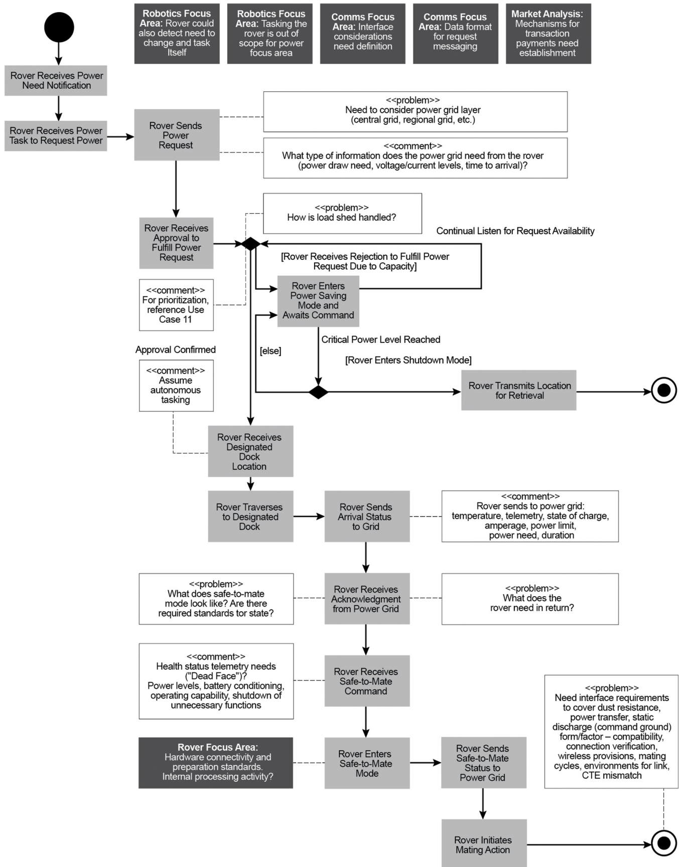
Figure 22.1. Example of rover use case activity diagram developed within LOGIC
