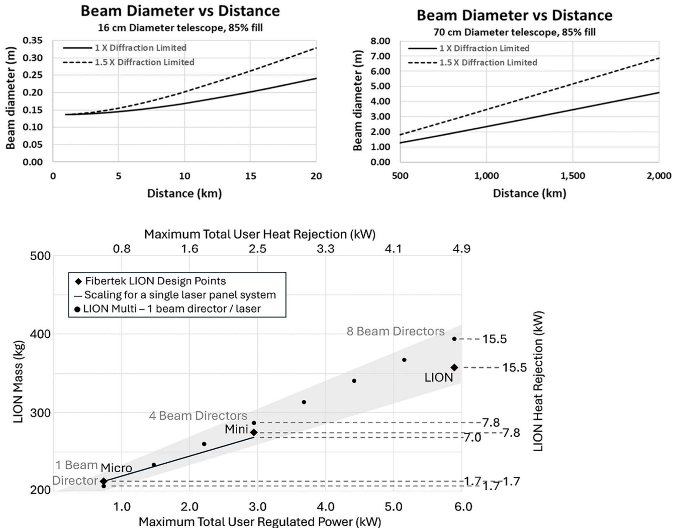
Figure 4.4. (Upper left) Laser beam diameter vs. range assuming a 16 cm telescope. (Upper right) Laser beam size vs. range for a 70 cm telescope in low lunar orbit (LLO) to the lunar surface. (Lower panel) LION mass vs. maximum total user regulated power and heat rejection for a range of LION terminals. The scaling of a single laser LION terminal is also shown. [Credit: Fibertek]
