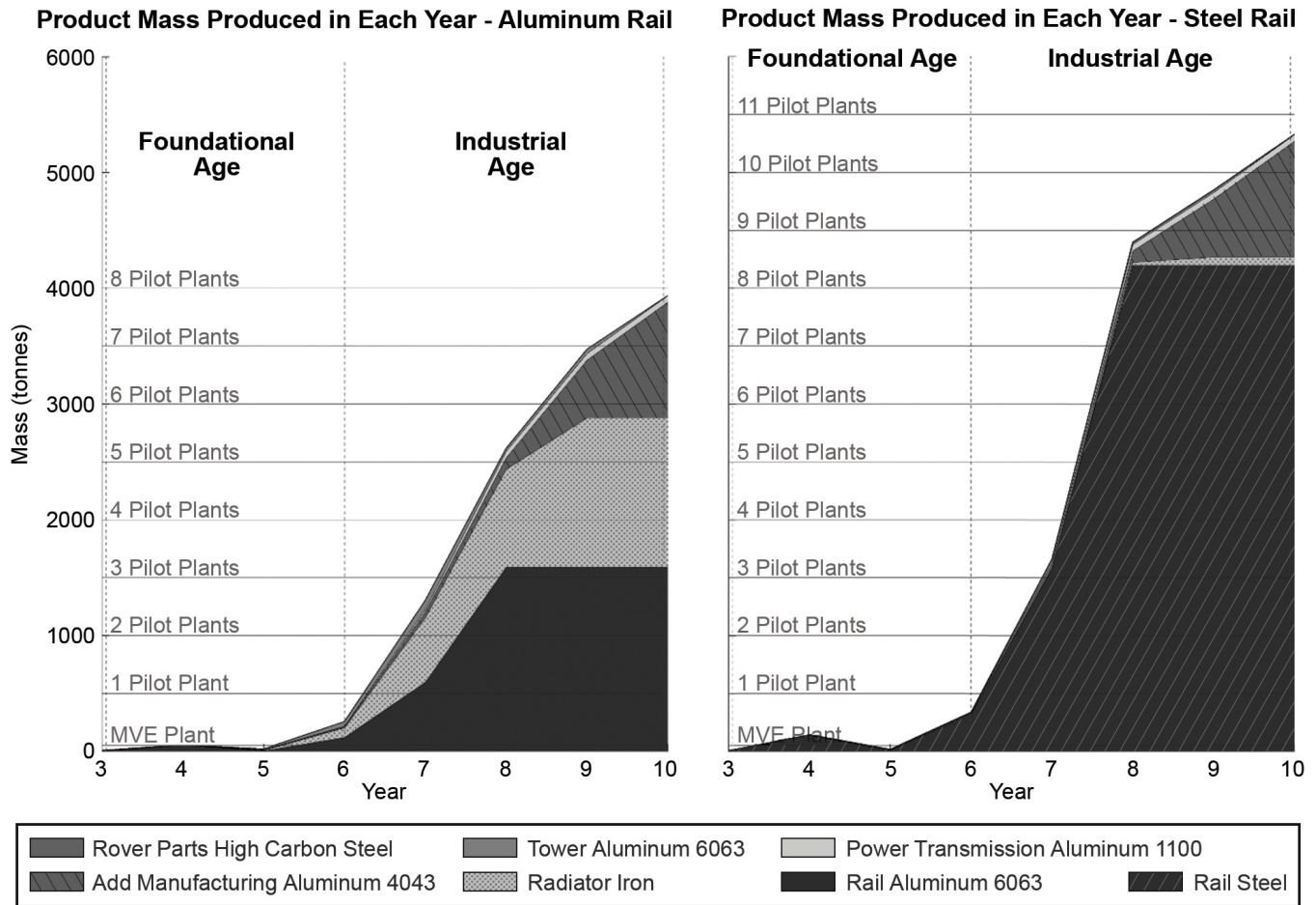
Figure 6.6. Foundry product production by mass versus year; (left) aluminum rail and (right) steel rail.
