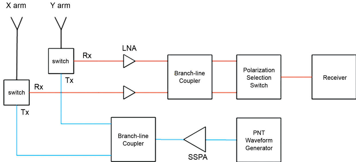
Figure 7.2. RF system architecture capable of switching between PNT transmit and SD receive functions. [Credit: Redwire Space]
