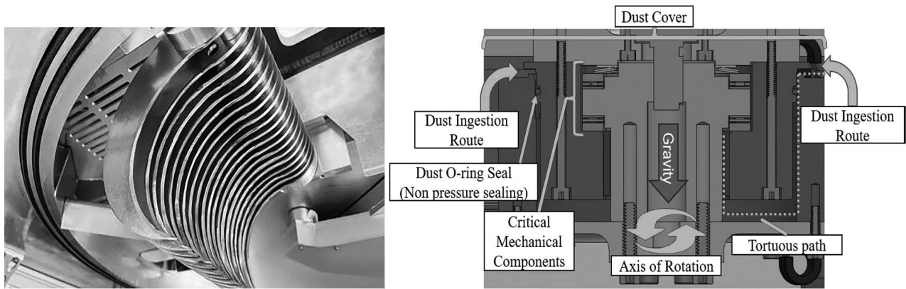
Figure 5.4. (Left) Rake design to separate the slag from the unprocessed regolith. (Right) Rotating joint within a prototype carbothermal reactor that uses a labyrinth pathway to protect against dust. [Credit: Sierra Space]
