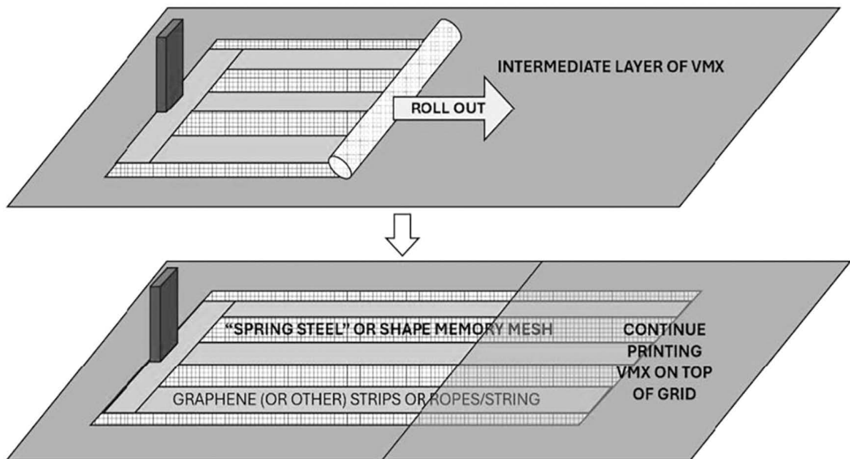
Figure 11.5. Construction details of conductive thermal battery. [Credit: ICON]
