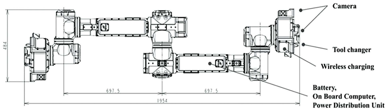
Figure 8.1. The Inchworm robot. [Credit: GITAI]
