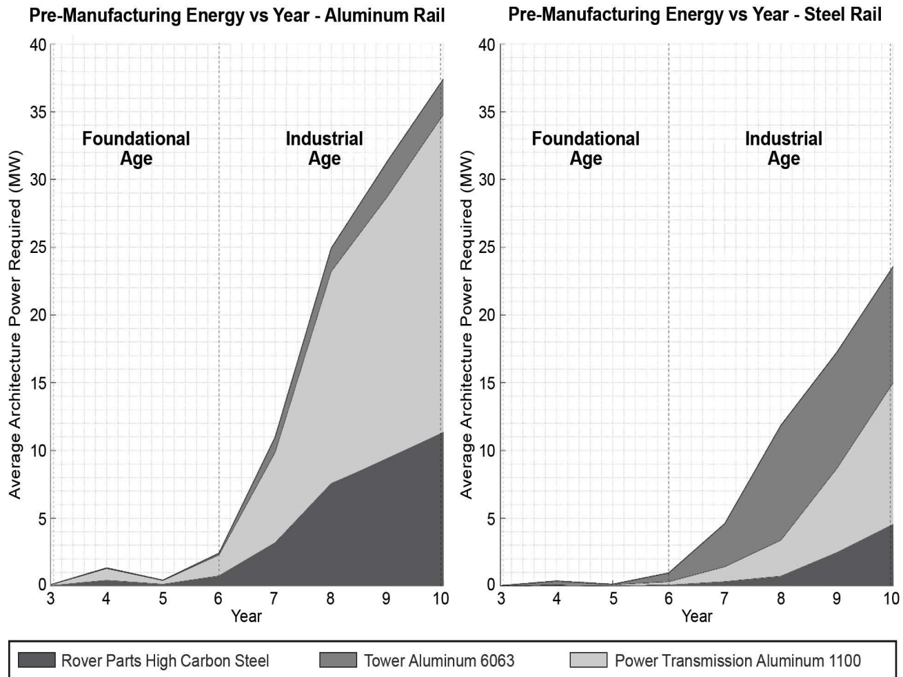
Figure 6.7. Energy consumption for ISRU metal refinement by year. (Left) aluminum rail and (right) steel rail.
