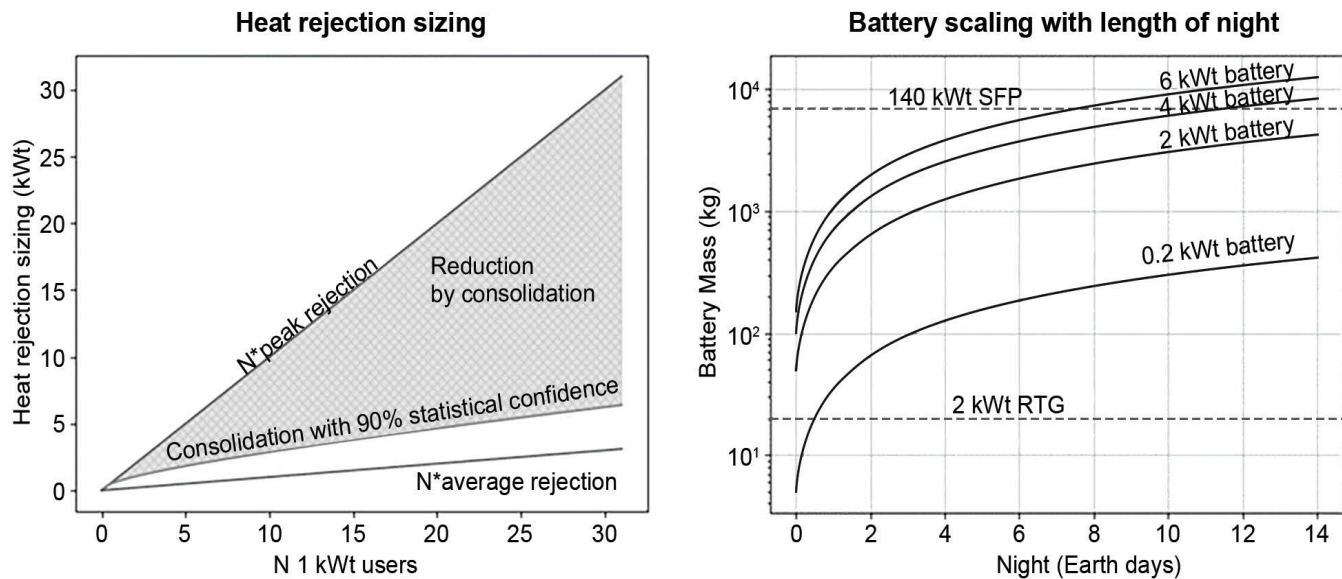
Figure 11.2. (Left) Benefit of consolidation. Plot shown with 1 \text{kW}_t users with a ten-to-one peak to average duty cycle. Consolidation line is the expected peak sum with 90 percent confidence using a one-tailed student t-test with a peak of two standard deviations from average. (Right) Battery mass as a function of lunar night length. Masses of surface fission power 7 and a radioisotope thermoelectric generator are shown for comparison. [Credit: Honeybee Robotics]
