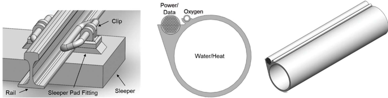
Figure 12.3. (Left) The integrated rail design, and its four main components. (Middle and right) Additional service infrastructure including power/data wired transmission, a water/heat pipeline, and an oxygen pipeline. [Credit: Northrop Grumman]
