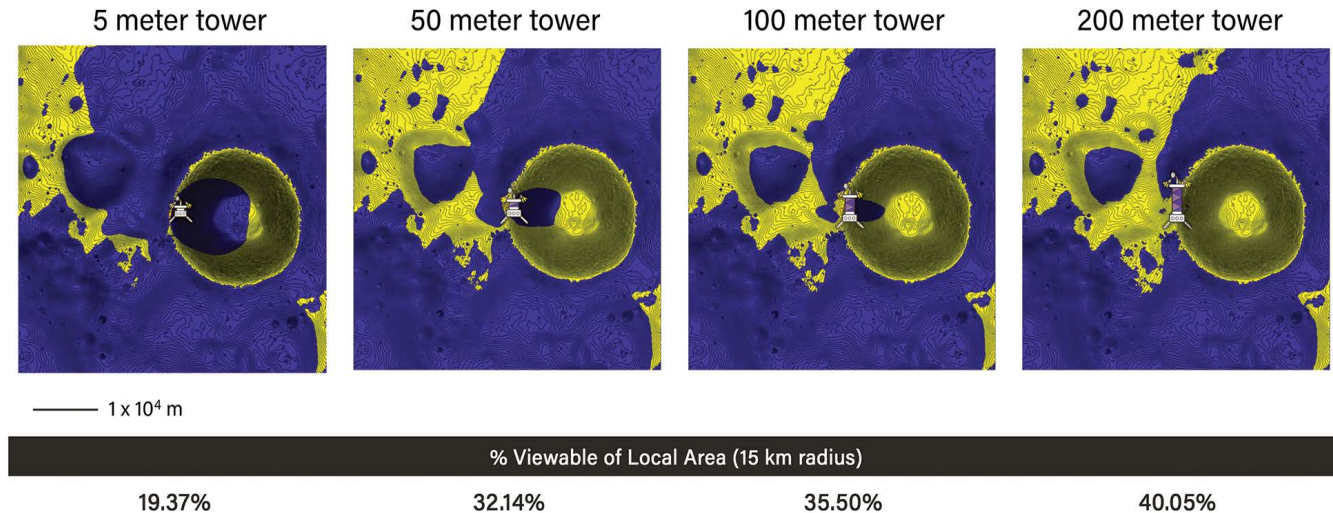
Figure 4.5. Viewshed for four selected heights of tower atop which an OWPT unit could be hosted. [Courtesy Honeybee Robotics]
