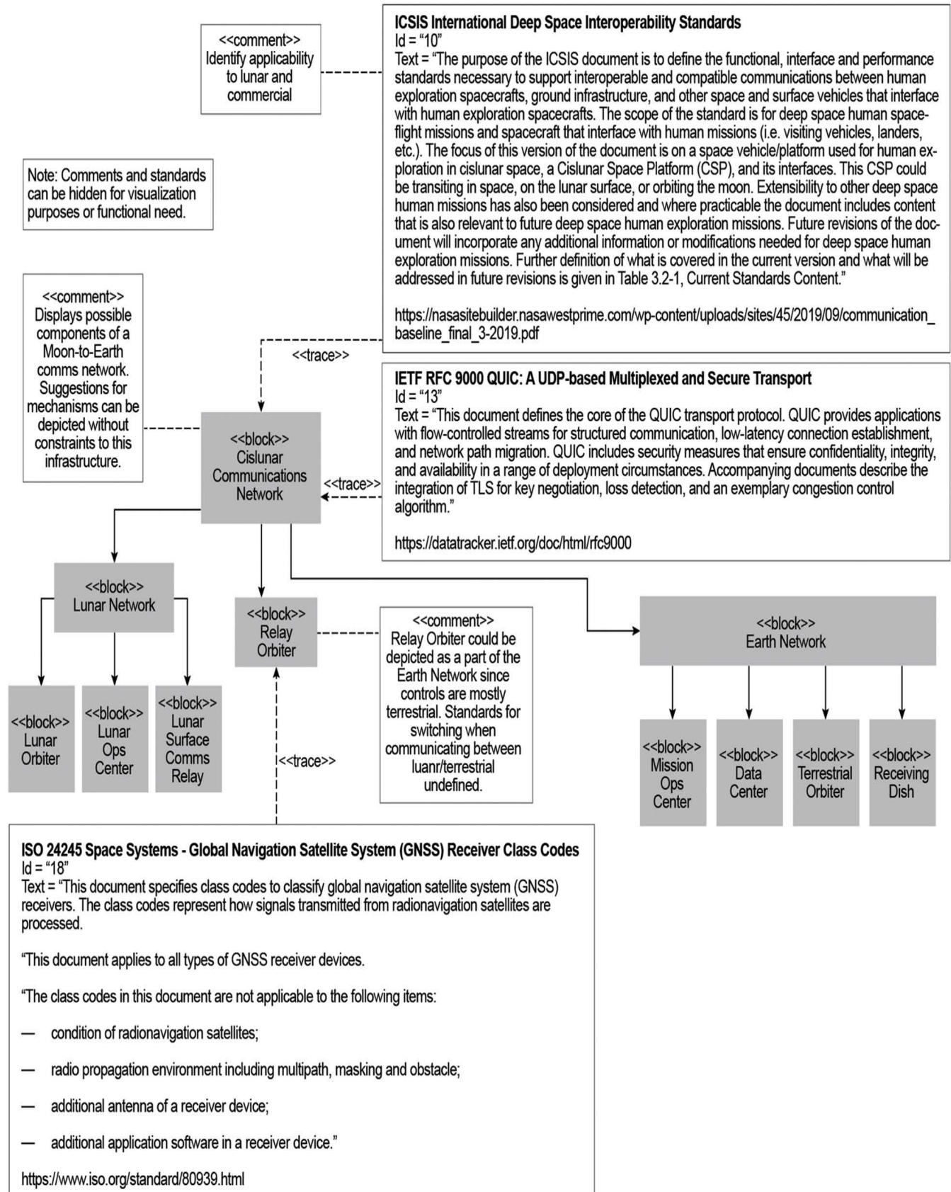
Figure 22.3. Communications and PNT block definition diagram and notional mapping of standards to block elements
