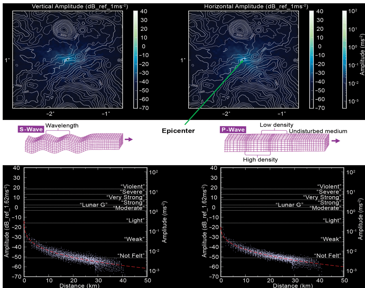
Figure 10.2. (Top) Heat map of S- and P-wave amplitude as a function of distance from the epicenter of crash anomaly. (Bottom) Amplitude of S- and P-waves as a function of distance from the epicenter of crash anomaly. [Credit: Honeybee Robotics]
