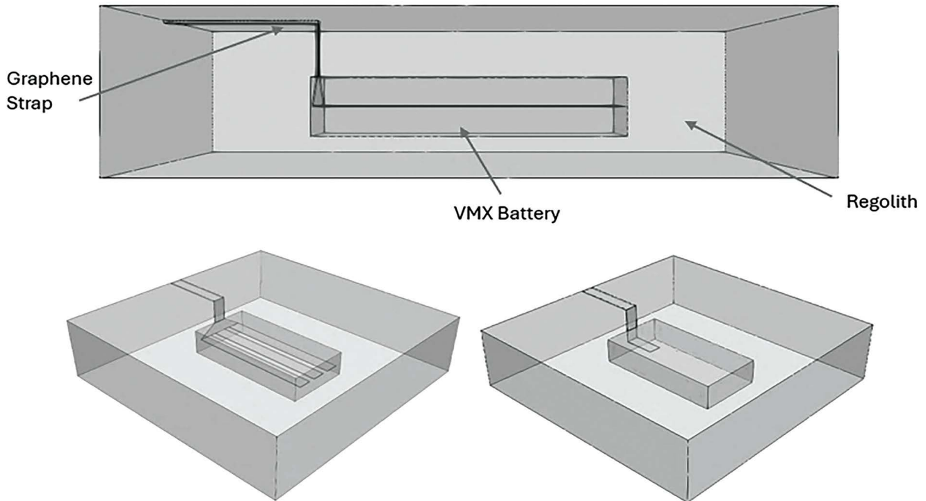
Figure 11.7. System configuration for proposed conductive battery. Graphene was chosen for very high thermal conductivity and space flight applications in the form of thermal straps. The graphene strap to the left provides a “connector” for any device that needs to dump thermal energy. The thermal straps are placed and incorporated into the VMX melt to form a robust conductive interface. The variant shown here on the lower left uses an array of thermal conductor “tendrils” embedded in the VMX battery to enhance bulk thermal conductivity. Bottom right of the image illustrates the device without the added tendrils. [Credit: ICON]
