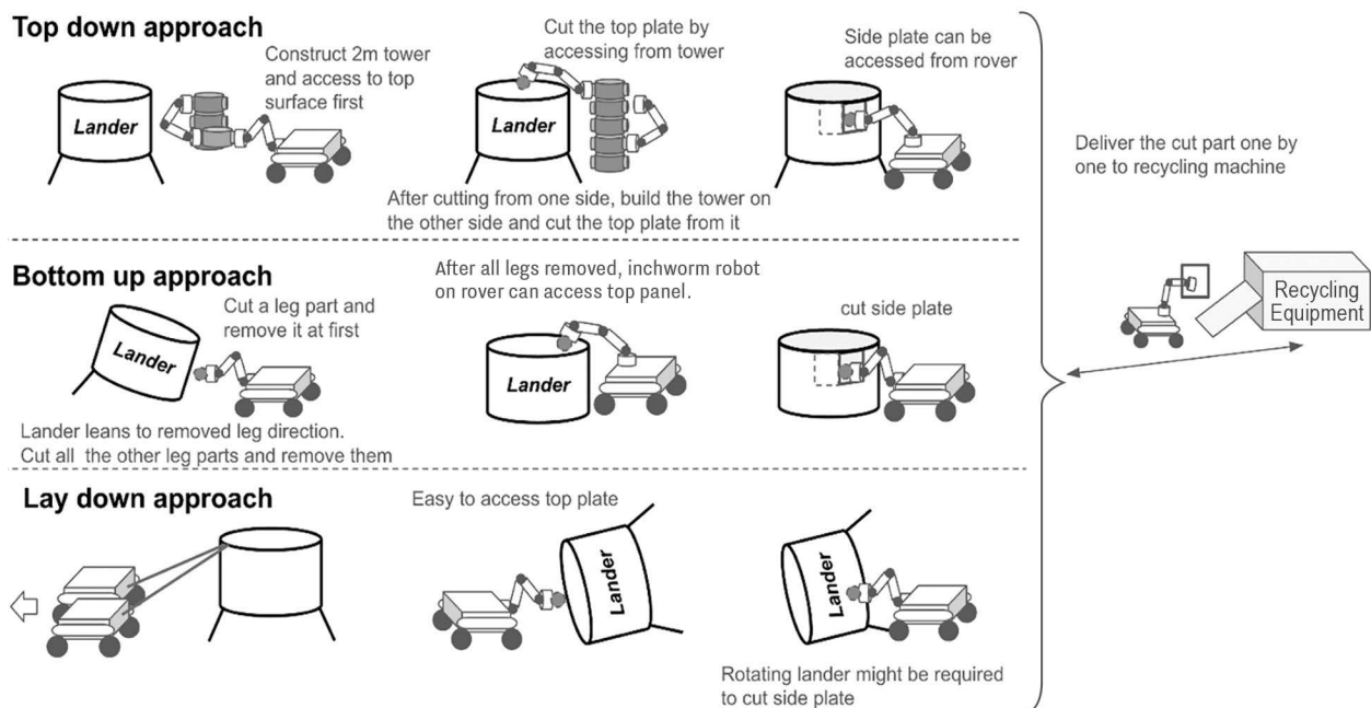
Figure 8.7. Use Case 3: Concept of disassembly of a lunar lander. [Credit: GITAI]
