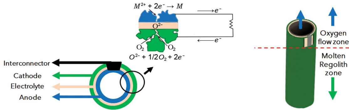
Figure 5.1. (Left) Cross section of a tubular cell. (Right) Top up view of tubular cell. [Credit: Helios Project Ltd.]
