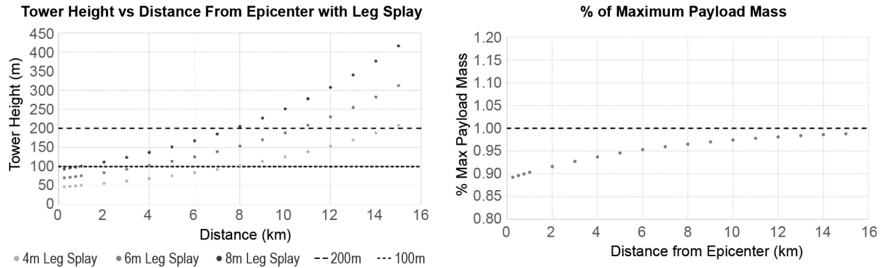
Figure 10.3. (Left) Maximum height for given leg splay (4 m, 6 m, 8 m) as a function of distance from epicenter. Primarily driven by P-waves, this shows that a standoff distance of 10 km for rocket landings should be sufficient to ensure no adverse interactions. (Right) Percentage total mass capacity for a system that has a requirement for surviving a crash anomaly. [Credit: Honeybee Robotics]
