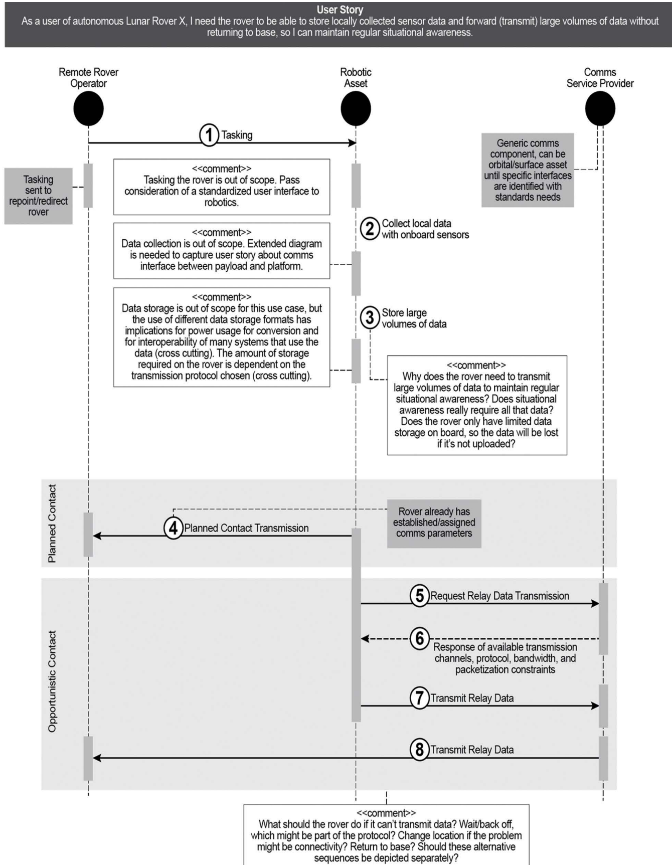
Figure 22.2. Example of a sequence diagram developed within LOGIC
