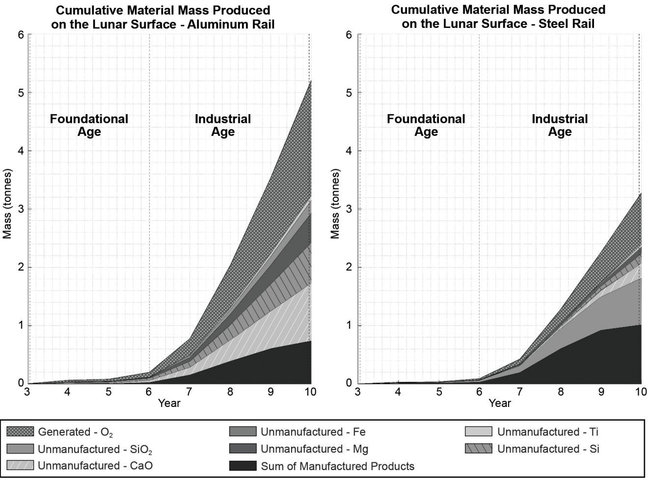
Figure 6.8. Cumulative material production. (Left) Aluminum rail; (Right) steel rail
