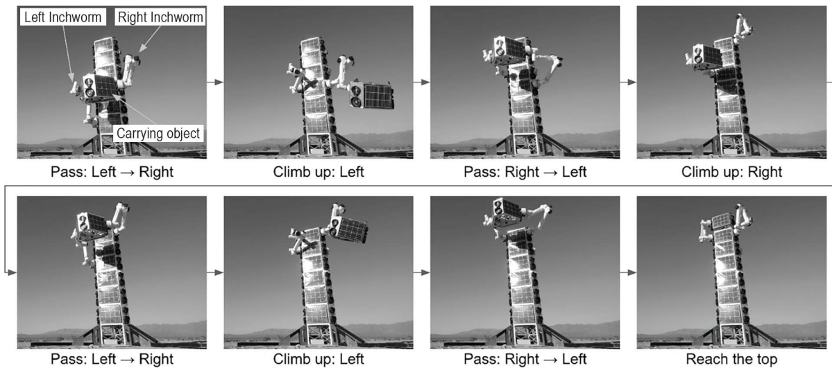
Figure 8.6. Real-world test of vertical logistics by relaying objects with multiple robots. [Credit: GITAI]
