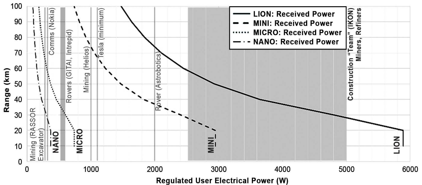
Figure 4.3. Range vs. maximum regulated electrical power provided to the user for LION Full, Mini, Micro, and Nano. Various surface capabilities and corresponding power requirements are overlaid. [Credit: Fibertek]
