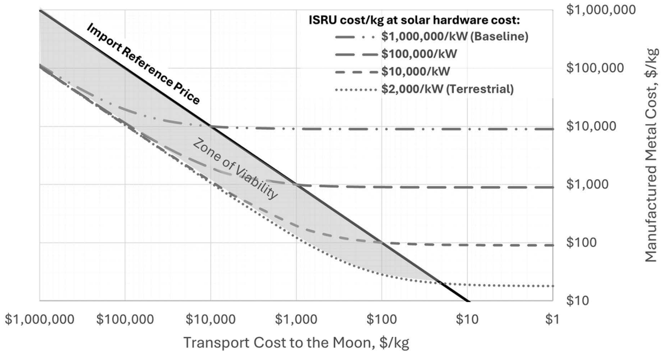
Figure 6.5. Cost of manufactured metal on the lunar surface, ISRU vs. import. [Credit: CisLunar Industries]
