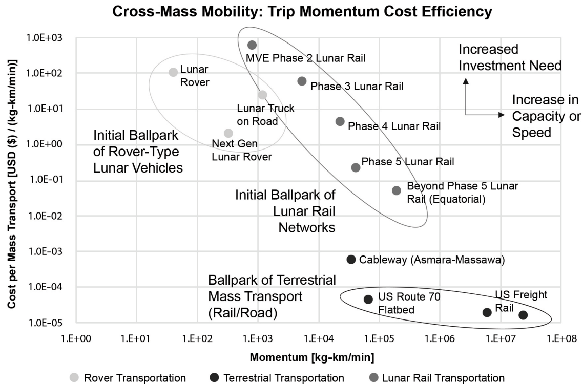
Figure 12.6. White space plot examining trip momentum cost efficiency for cross-mass mobility. [Credit: Northrop Grumman]
