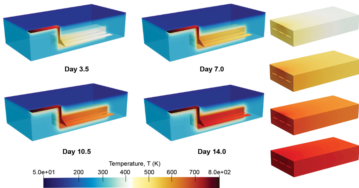
Figure 11.10. Graphene tendrils configuration under constant 800 K input temperature condition. [Credit: ICON]
