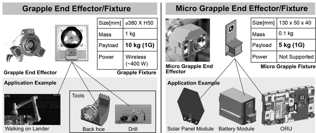
Figure 8.2 Specification of grapple fixtures. [Credit: GITAI]
