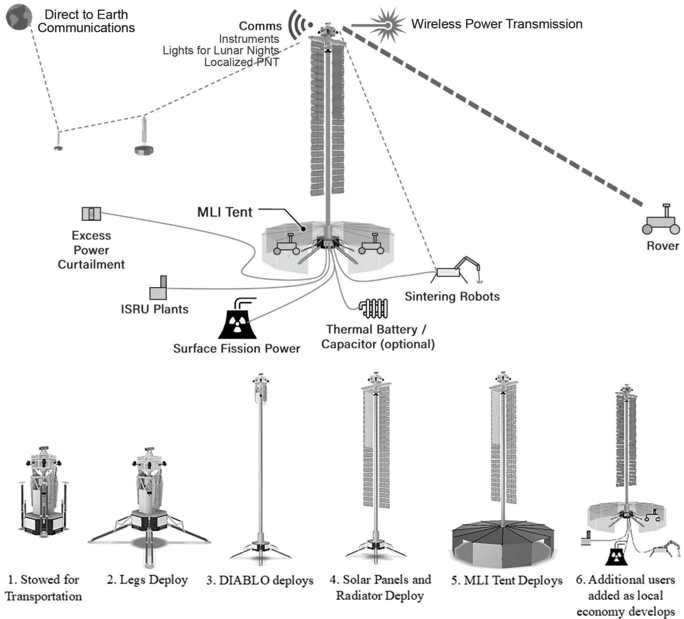
Figure 11.1. (Upper) Lunar Oasis utilizes a LunarSaber tower to create a centralized hub of services for users. (Lower) Lunar Oasis deployment concept of operations. [Credit: Honeybee Robotics]
