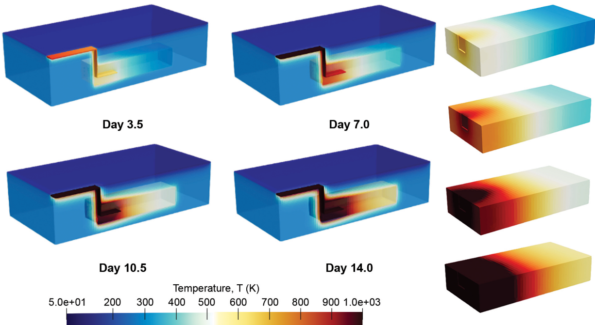
Figure 11.9. Graphene strap configuration under constant 200 W input power condition. [Credit: ICON]
