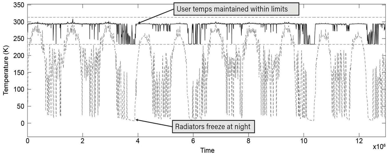
Figure 11.3. Lunar Oasis manages the temperatures of thirty users with consolidated thermal management. Individual management would require 2.1 times more radiator area for the same performance. [Credit: Honeybee Robotics]
