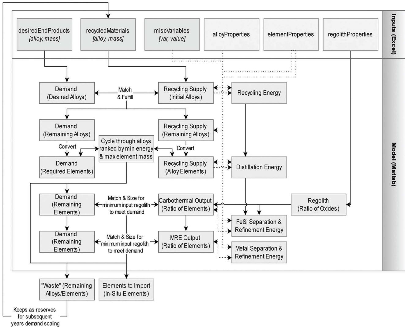
Figure 6.4. Metal framework energy-mass model. [Credit: CisLunar Industries]
