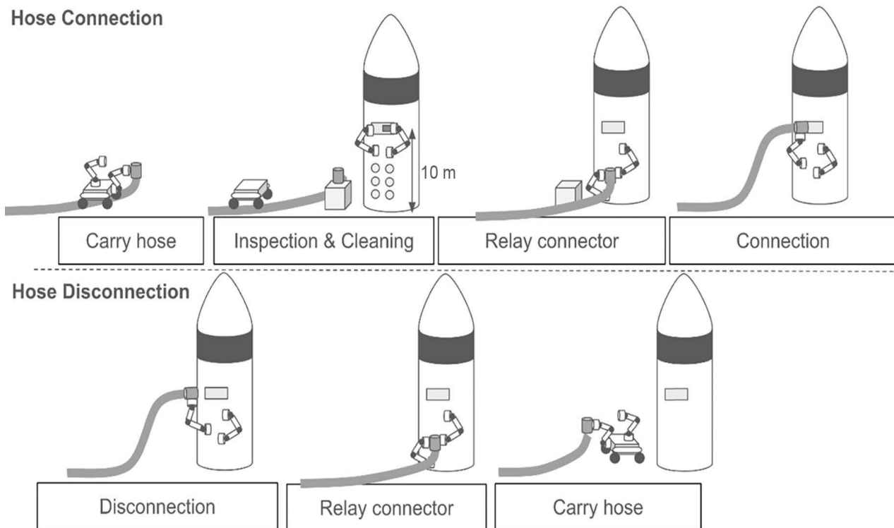
Figure 8.5. Use Case 2: Concept of operations of refueling LOX for a launcher: Inchworm and Mover robots work in tandem to conduct the required tasks. [Credit: GITAI]
