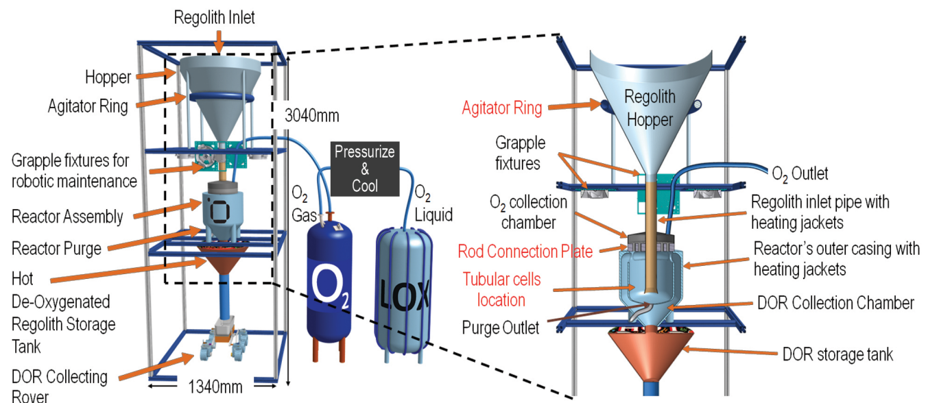
Figure 5.2. (Left) MVE System concept for lunar oxygen. (Right) MVE reactor cross section. [Credit: Helios Project Ltd.]
