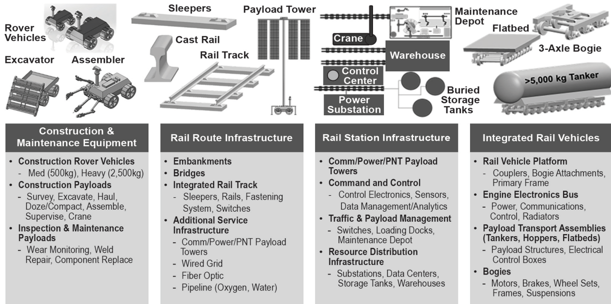
Figure 12.1. Lunar Rail Network Infrastructure product data structure. [Credit: Northrop Grumman]
