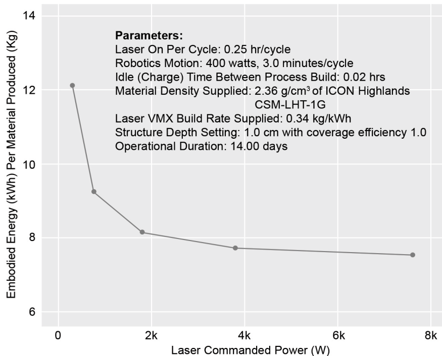
Figure 9.3. Laser VMX embodied energy (kWh) per kg material produced vs. laser commanded power (W). [Credit: ICON]
