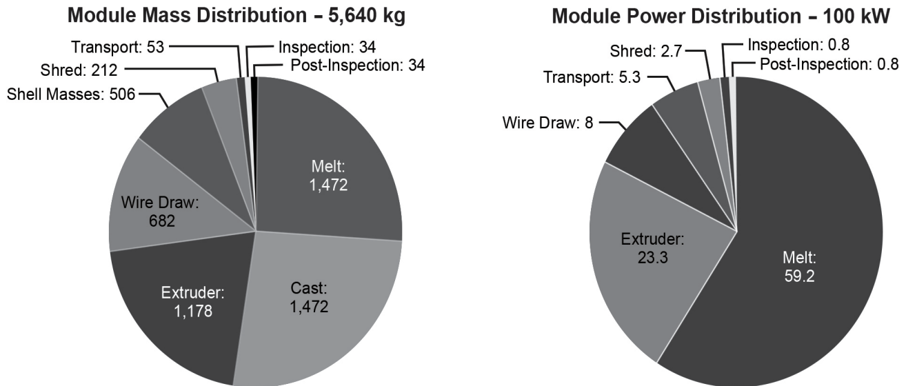
Figure 6.3. Pilot foundry mass and power across modules. [Credit: CisLunar Industries]
