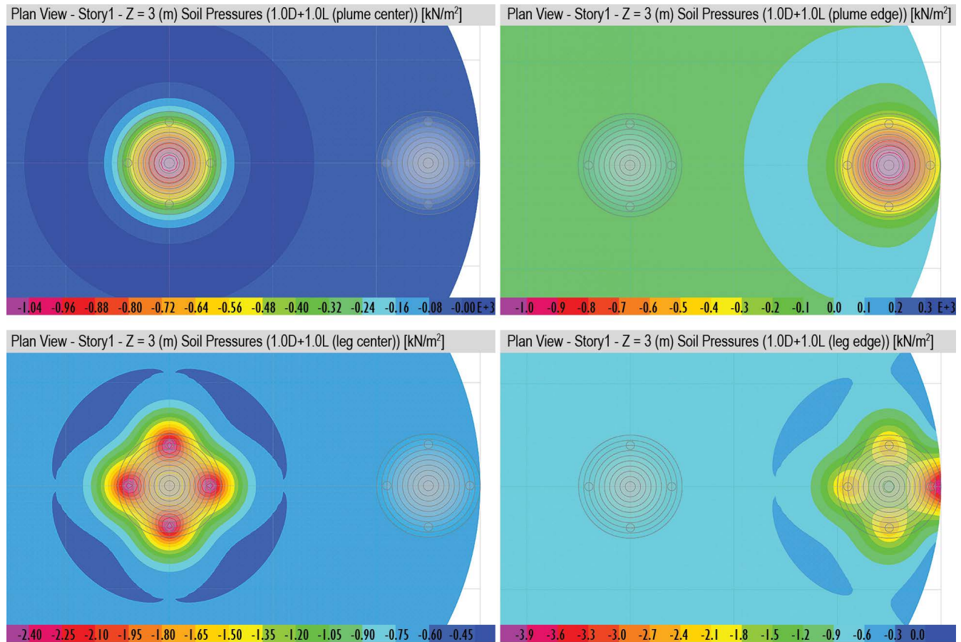
Figure 9.1. Example soil pressure results for 150 mm pad with 90 percent D_r subgrade. Secondary landing loading shown in gray is for context only and is not applied to the soil conditions. [Credit: ICON]
