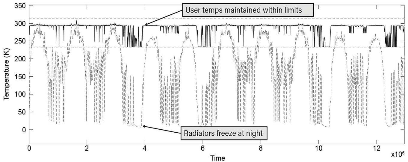
Figure 11.3. Lunar Oasis manages the temperatures of thirty users with consolidated thermal management. Individual management would require 2.1 times more radiator area for the same performance. [Credit: Honeybee Robotics]
