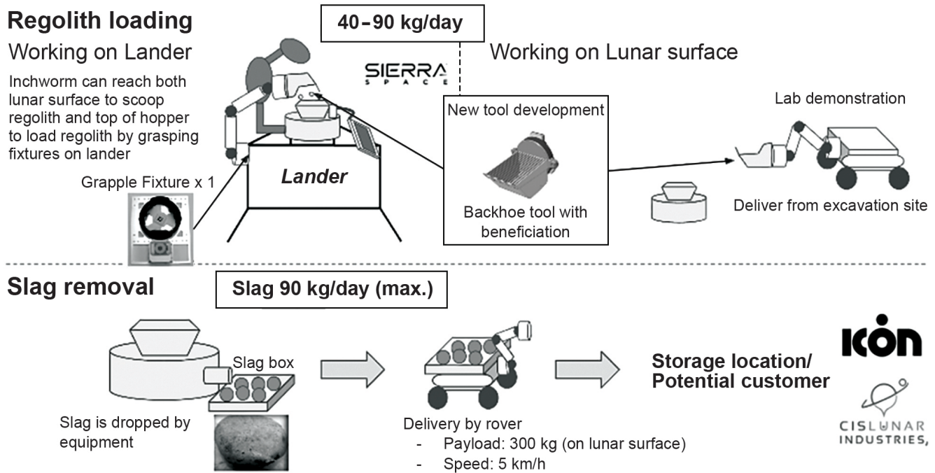
Figure 8.4. Use Case 1, Concept of operations for RaaS-centered ISRU construction and operation, part 2: (top) For regolith loading, the Inchworm can reach both the lunar surface to scoop regolith and the top of the hopper to load the regolith, using grasping fixtures on the lander. (Bottom) For slag removal, the slag dropped by equipment is delivered by Mover robot to a storage location or a potential customer. ICON and CisLunar Industries are notional partners in this process. [Credit: GITAI]
