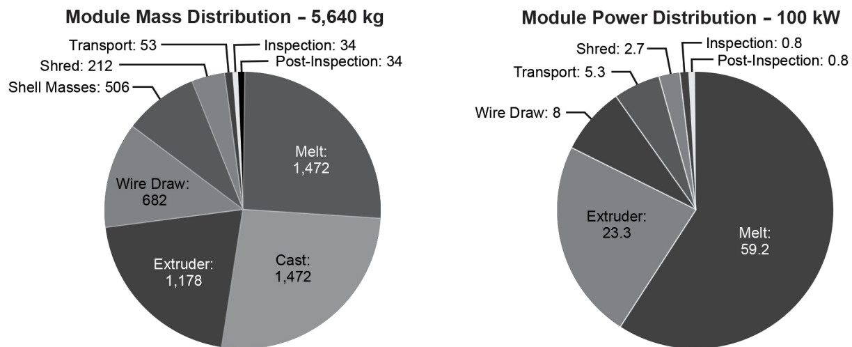
Figure 6.3. Pilot foundry mass and power across modules. [Credit: CisLunar Industries]
